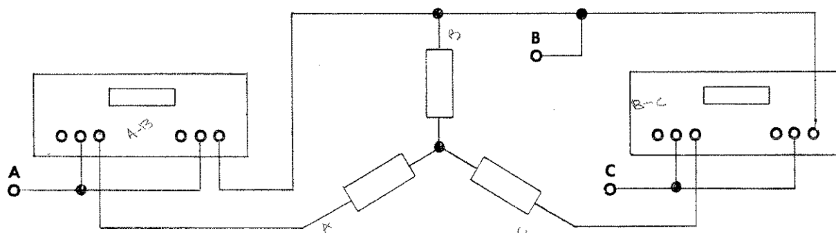
Two Wattmeter/Three Wire Case. (delta or Y Load)
