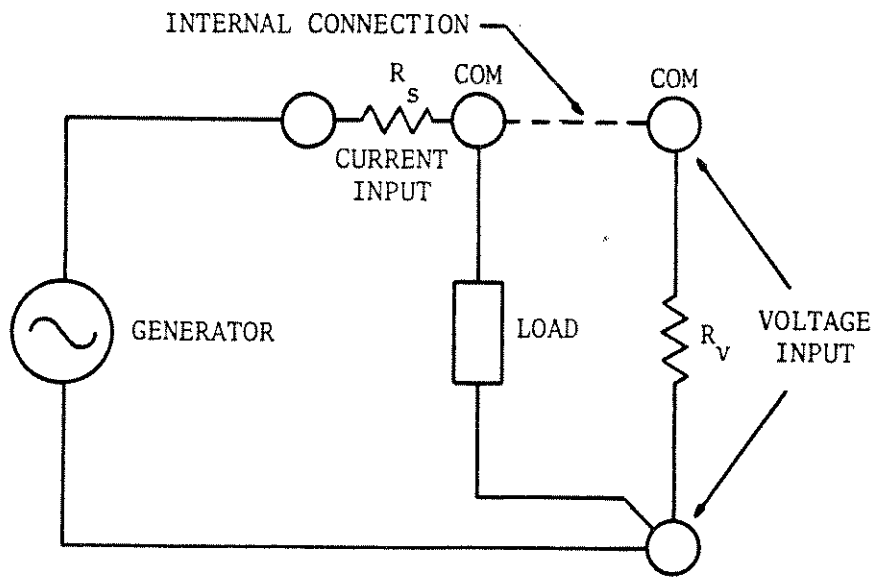
Shunt High Wattmeter Connection. Meter Reading is Negative and Requires a Correction of V^2/R_v .
