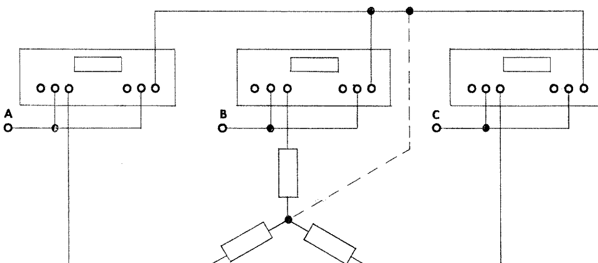
Three Wattmeter/Three or Four Wire Case.
